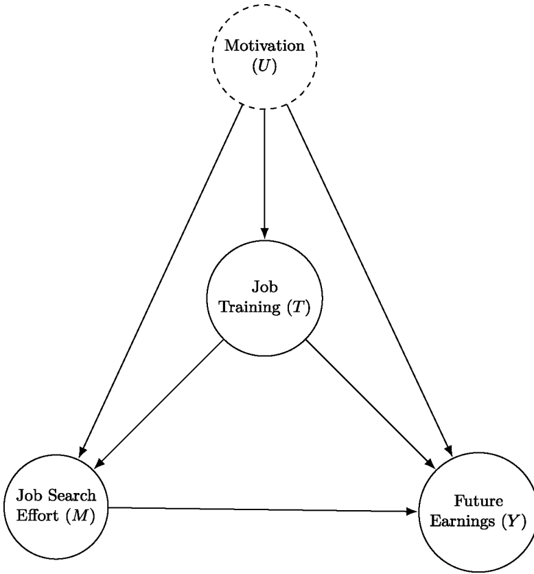
Fig. 4 Mediation with Unmeasured Confounding: Motivation ( U ) affects Job Training ( T ), Job Search Effort ( M ), and Future Earnings ( Y )
