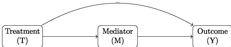
Fig. 3 Causal diagram illustrating mediation
