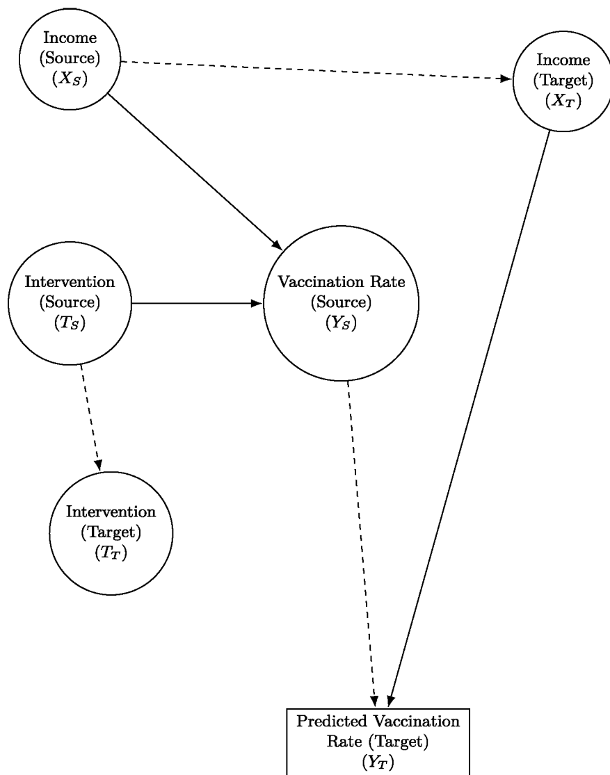
Fig. 8 Transportability Example: Predicting Target Vaccination Rate ( Y_T ) from Source Domain ( T_S , X_S , Y_S ) using shared covariates and structural similarities. Dashed arrows represent domain transport mappings
