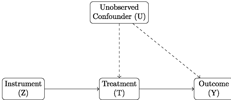
Fig. 2 Causal diagram illustrating an instrumental variable
