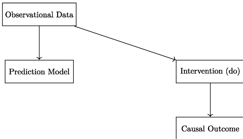
Fig. 1 Visualizing prediction versus causation
