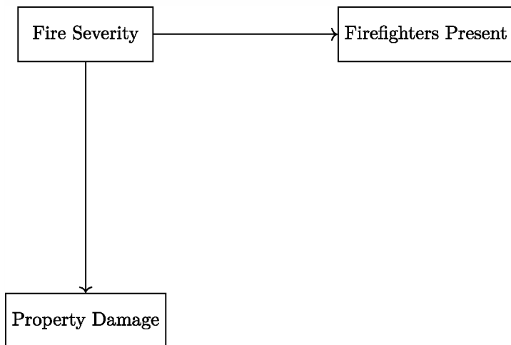
Fig. 3 Correlation versus causation
