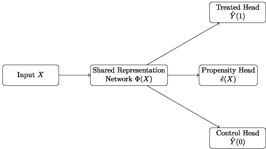
Fig. 1 DragonNet Architecture: Shared representation network with heads for treated outcome, control outcome, and propensity score
