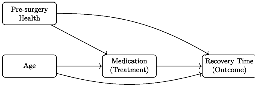
Fig. 4 Causal diagram: effect of medication on recovery time, with age and pre-surgery health as confounders
