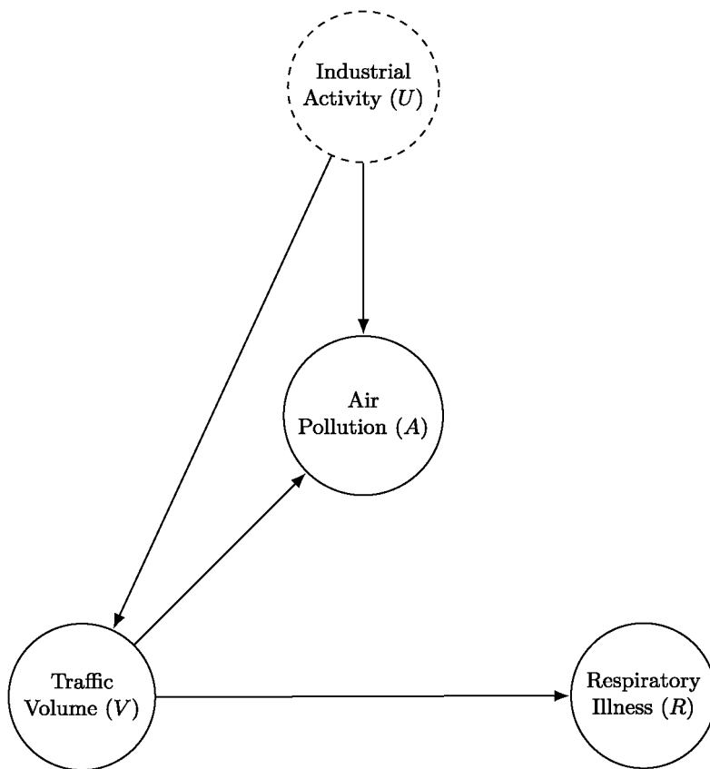
Fig. 6 Causal Discovery with a Latent Confounder: Industrial Activity ( U ) affects both Air Pollution ( A ) and Traffic Volume ( V ); V affects both A and Respiratory Illness ( R )
