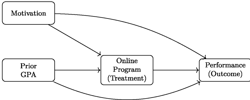
Fig. 2 Causal diagram: online program effect on performance, with prior GPA and motivation as confounders
