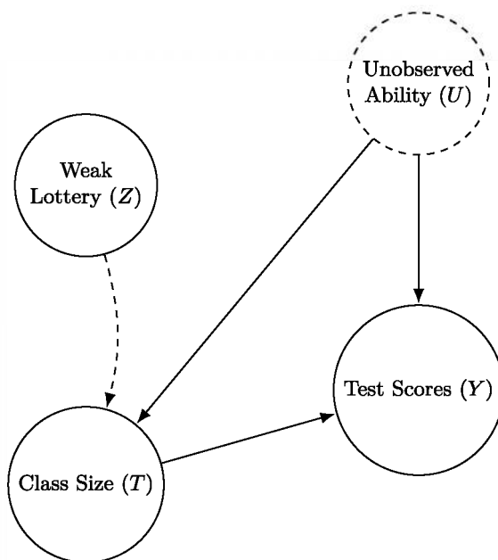
Fig. 2 Weak Instrument Scenario: the lottery instrument ( Z ) has a weak causal effect on class size ( T )
