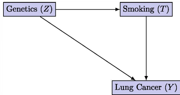
Fig. 1 Causal graph: Genetics influence smoking, influencing lung cancer
