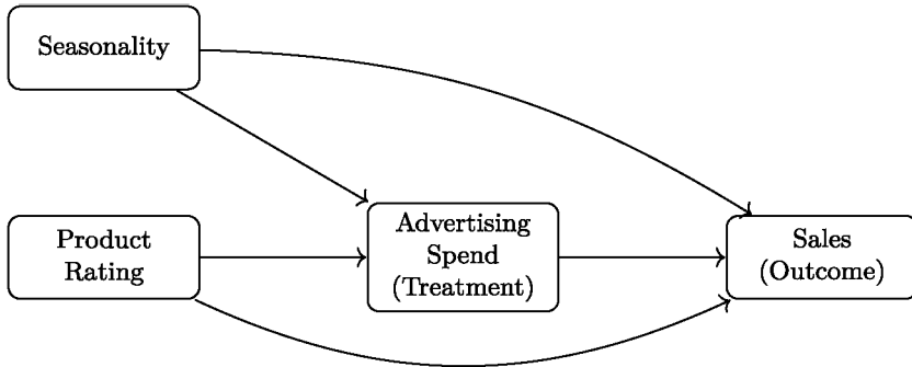
Fig. 3 Causal diagram: effect of advertising spend on sales, with seasonality and product rating as confounders
