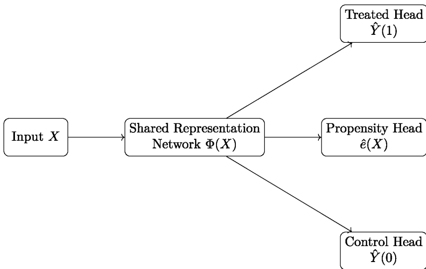
Fig. 3 DragonNet Architecture: outcome prediction and propensity score estimation with targeted regularization
