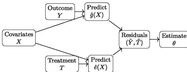
Fig. 4 Double Machine Learning pipeline: nuisance estimation followed by residual regression
