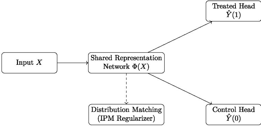
Fig. 2 CFRNet Architecture: TARNet plus distribution matching using an Integral Probability Metric (IPM) to balance representations
