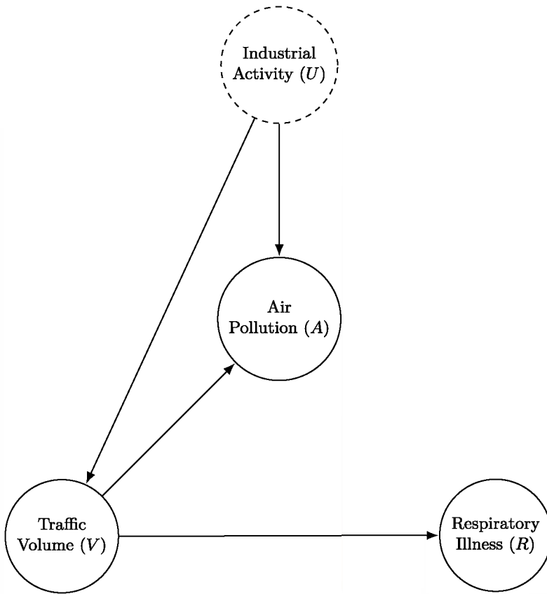
Fig. 7 Causal Discovery with a Latent Confounder: Industrial Activity ( U ) affects both Air Pollution ( A ) and Traffic Volume ( V ); V affects both A and Respiratory Illness ( R )
