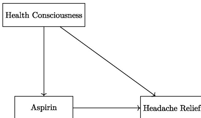
Fig. 2 Causal graph visual representation
