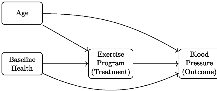
Fig. 1 Causal diagram: effect of an exercise program on blood pressure, with age and baseline health as confounders
