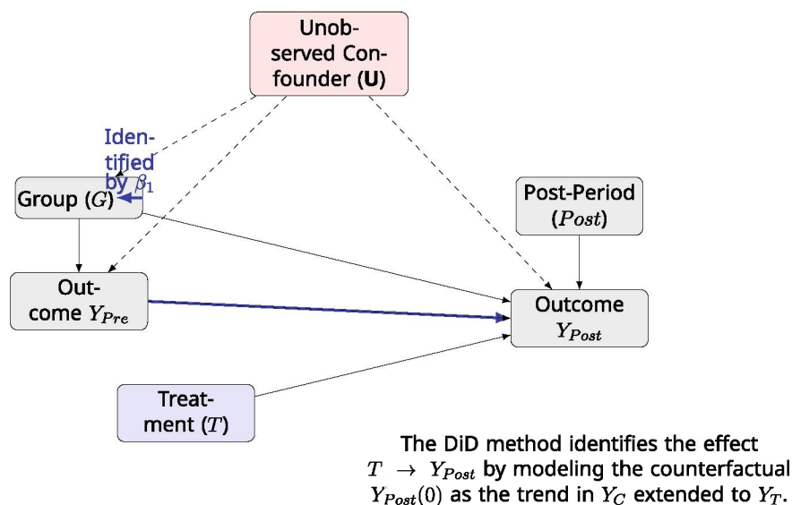
Fig. 9 Causal Diagram for a DiD Setup
