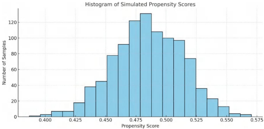
Fig. 2 Histogram of simulated propensity scores
