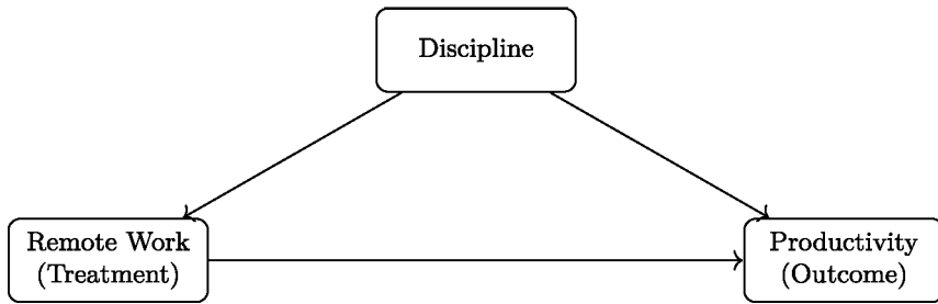
Fig. 5 Causal diagram: effect of remote work on productivity, with discipline as a confounder
