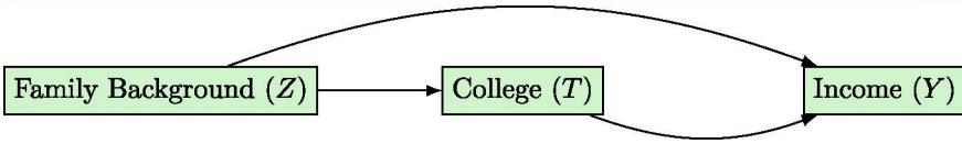
Fig. 4 Causal graph for education ( T ) and income ( Y ), with family background ( Z ) as confounder
