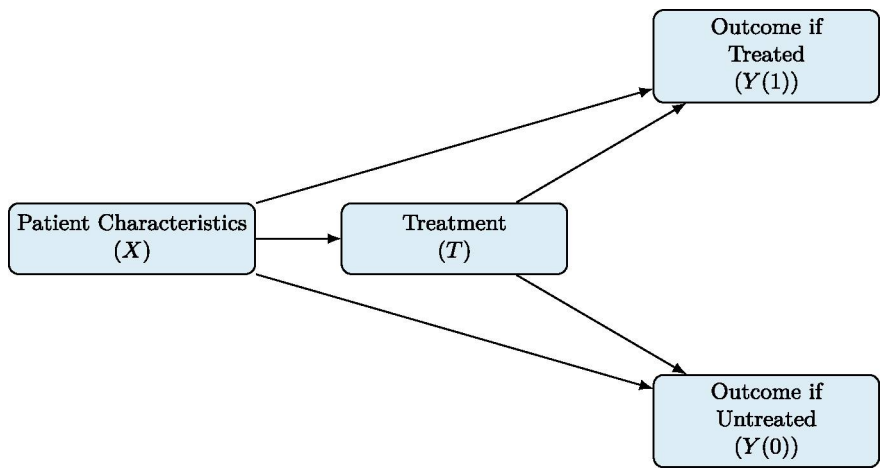
Fig. 5 Causal diagram showing counterfactual structure: only one of Y(1) or Y(0) is observed
