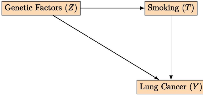
Fig. 2 Observational system: natural pathways from Z to T and Y exist
