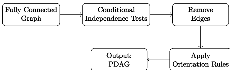
Fig. 1 Flow of the PC algorithm for causal discovery
