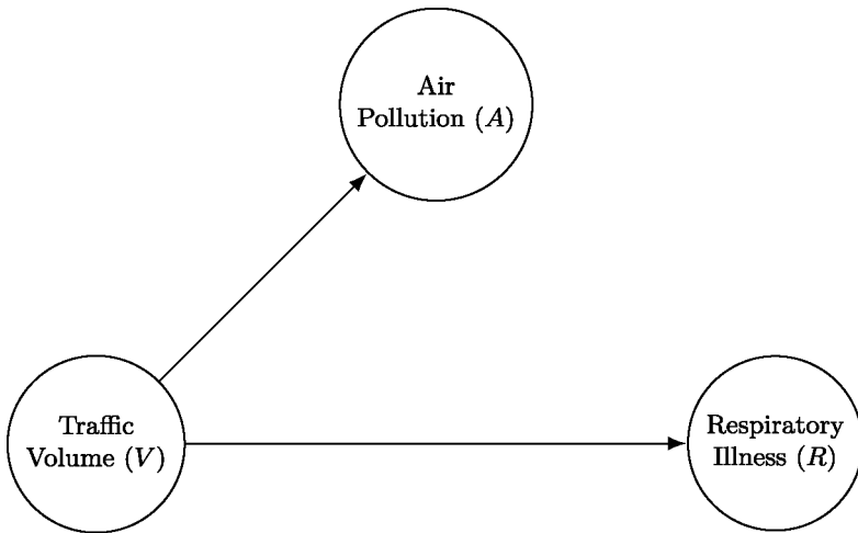
Fig. 5 Causal Discovery Example: Traffic Volume ( V ) affects both Air Pollution ( A ) and Respiratory Illness ( R )
