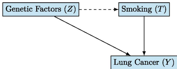
Fig. 3 Interventional system: Intervention breaks the natural path Z \rightarrow T
