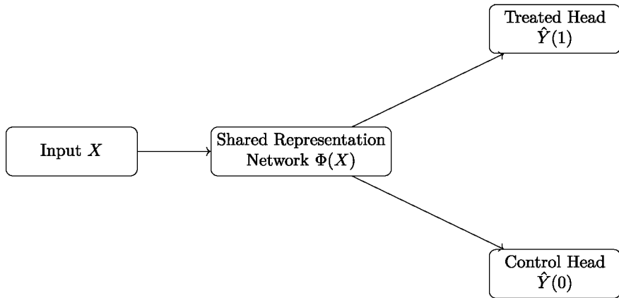
Fig. 1 TARNet Architecture: a shared representation network followed by two treatment-specific heads
