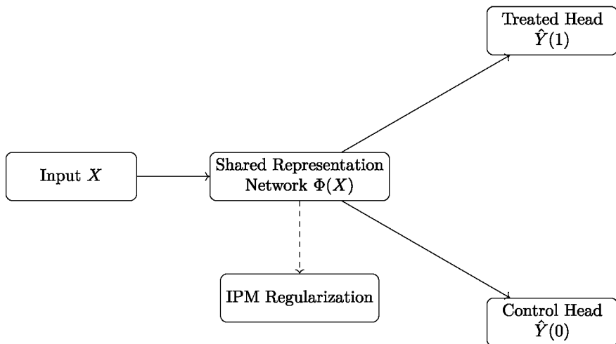
Fig. 1 CFRNet Architecture: shared representation network with treatment-specific heads and a balancing regularizer
